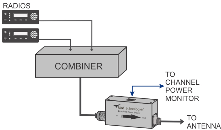
Figure 2 Connection Diagram
