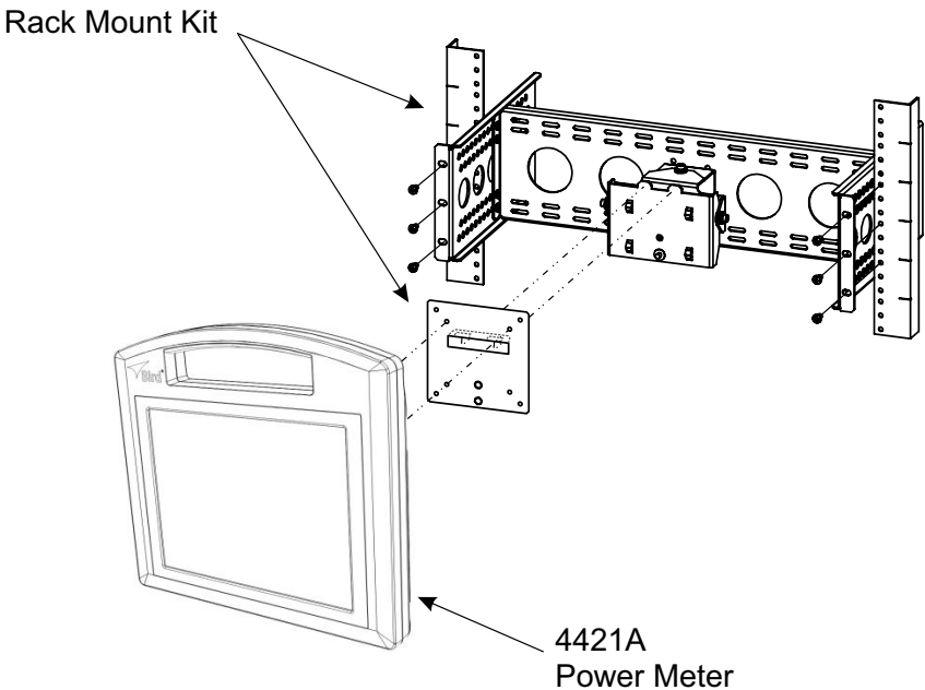
Figure 1 Rack Mount Kit
