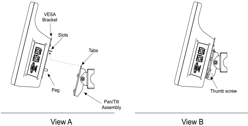
Figure 7 Attach 4421A to Rack Mount
