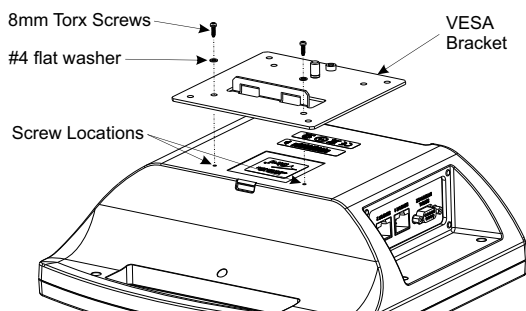
Figure 3 Attach VESA Bracket
