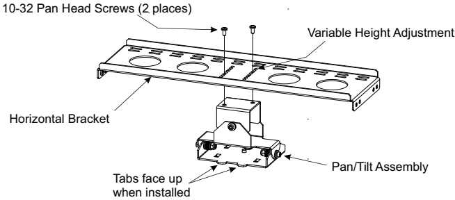
Figure 4 Pan/Tilt Assembly Attachment
