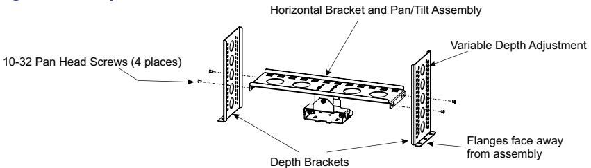
Figure 5 Depth Bracket Attachment
