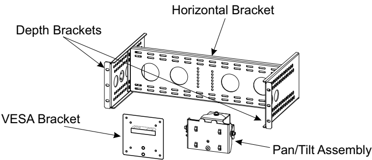
Figure 2 Rack Kit Contents
