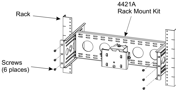
Figure 6 Rack Installation
