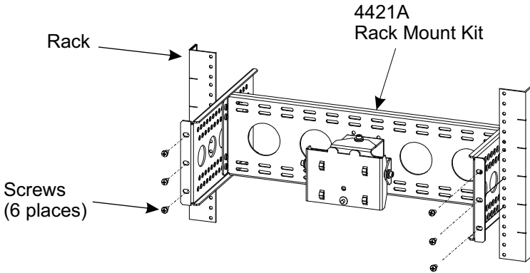
Figure 29 Rack Instalation
