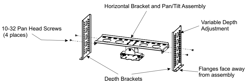
Figure 28 Depth Bracket Attachment
