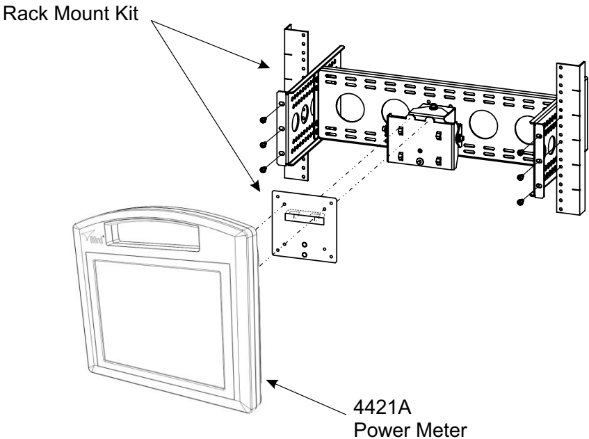
Figure 24 Rack Mount Kit
