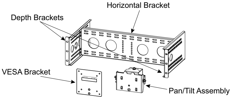
Figure 25 Rack Kit Contents
