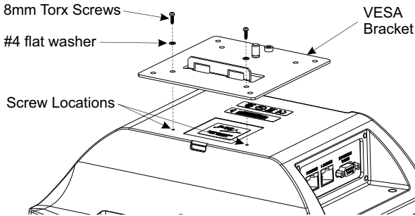
Figure 26 Attach VESA Bracket
