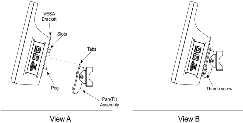
Figure 30 Attach 4421A to Rack Mount
