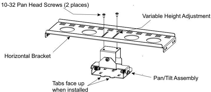
Figure 27 Pan/Tilt Assembly Attachment
