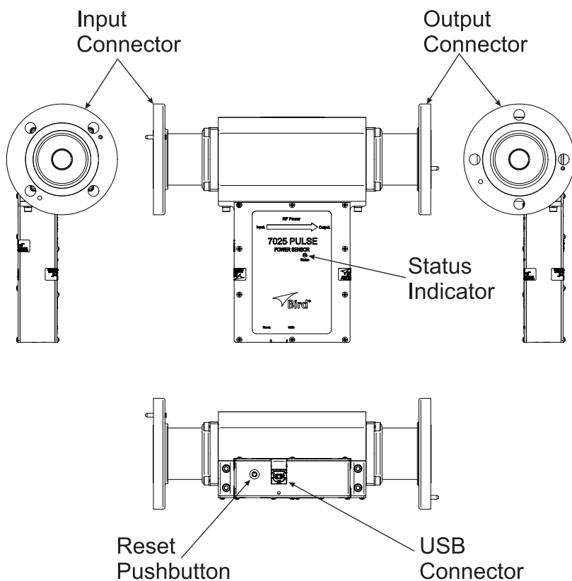
Figure 1 7025 Power Sensor
