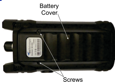
Figure 49 Battery Access
