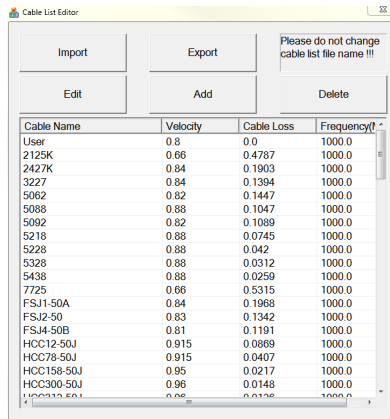
Figure 52 Cable List Editor
