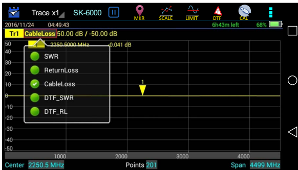
Figure 10 Selecting Cable Loss Measurement
